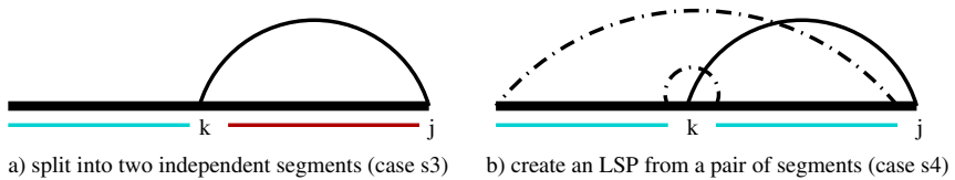
Fig. 4. Cases for matching segments
