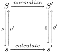
Fig. 4. Given that s = S \cdot \rho , it is convenient to consider S' , the sorted normalization of S , and s' = S' \cdot \rho : Proving that a legal scenario q' acting on s' is also an SBR scenario implies the uniqueness of the ancestor. Calculating s' directly from s enables the reconstruction of S in linear-time. Finally, finding an SBR scenario sorting s'|_N gives a legal scenario on s .
