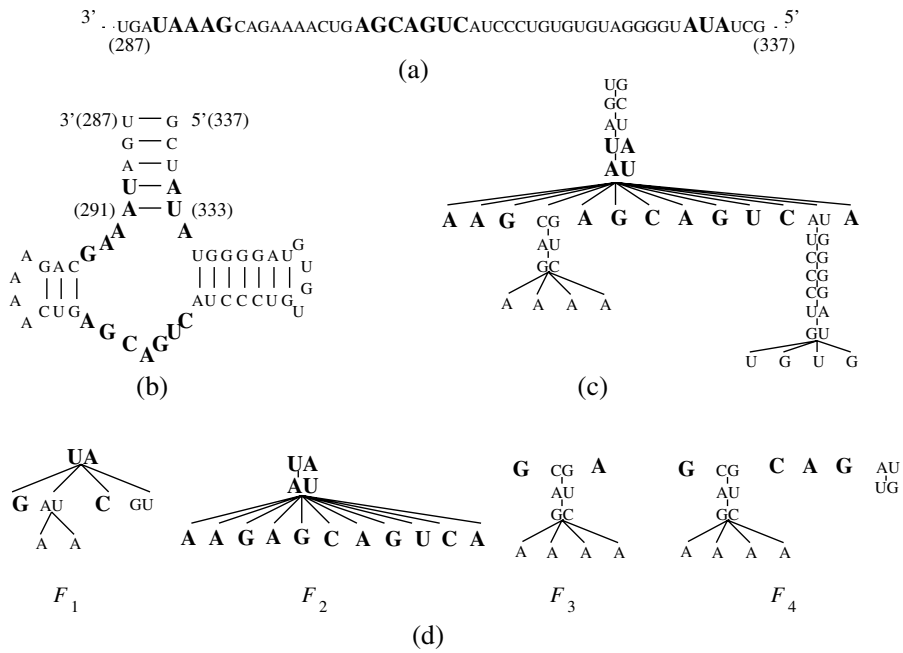
Fig. 1. (a) A segment of the primary structure of the cherry small circular viroid-like RNA molecule (accession number Y12833, GI:2347024) [10], (b) its secondary structure, (c) a forest representation F of the secondary structure (see, e.g., [4, 7, 11] for details), and (d) various types of subforests of F . The so-called Hammerhead motif [10], which corresponds to the pattern specified by subforest F_2 , is marked in bold.
