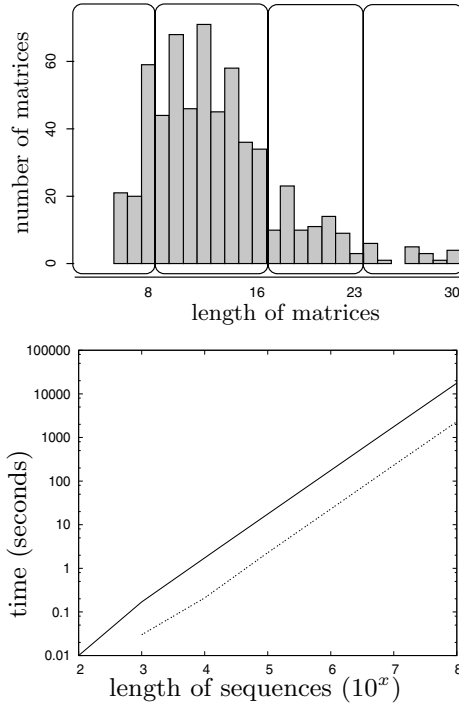
Fig. 4. The histogram represents the distribution of sizes of Transfac and Jaspard matrices (602 matrices in total). The optimal index table for this set of matrices is composed of four subtables: 1..8, 9..16, 17..23 and 24..30. The number of matrices in each subtable is respectively 602, 502, 100 and 20. After pruning with lemma 1, the corresponding average number of accesses is respectively 602, 216, 18 and 1. The second figure gives the computation time of our algorithm (dotted line) compared to the brute-force algorithm (solid line). The available memory size was 256MB. The second diagram shows that our algorithm is eight times faster than the brute-force one.
